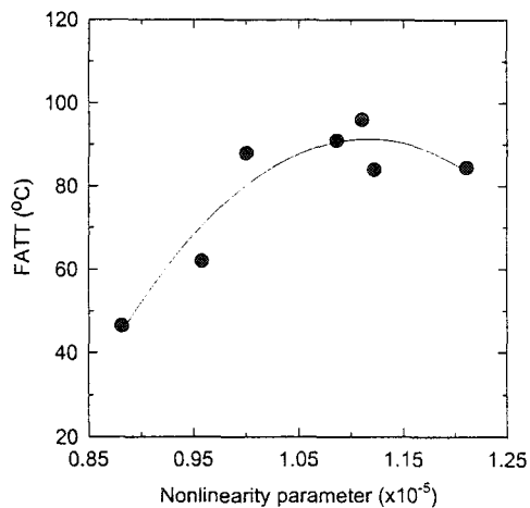
Fig. 6 Correlations between the nonlinearity parameter and the FATT
