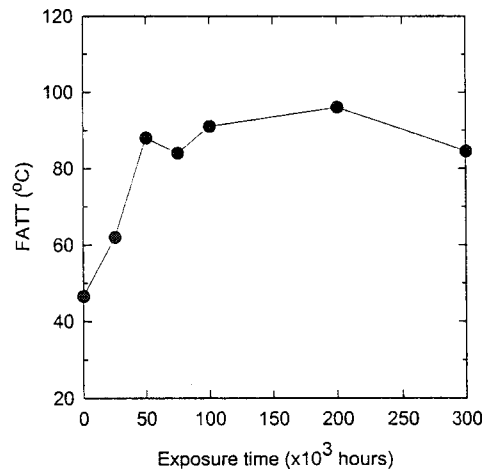
Fig. 3 Dependence of FATT on aging time
