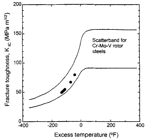
Fig. 5 Estimated fracture toughness based on the K_{Ic} versus excess temperature correlations and the K_{Ic} scatterband for retired CrMoV rotor steels
